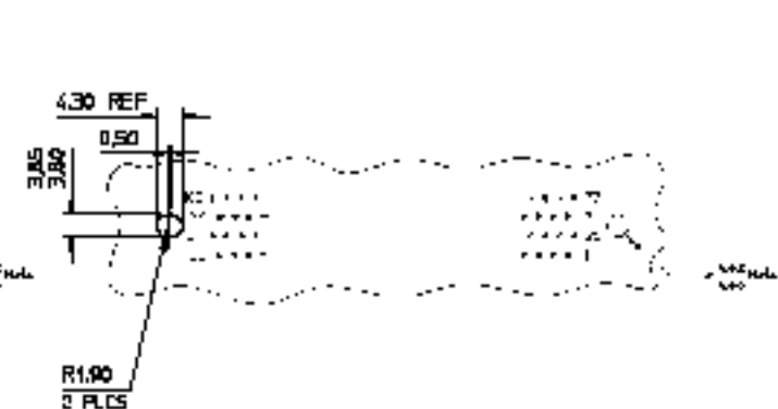
LAYOUT VIEWED FROM FEMALE SIDE
